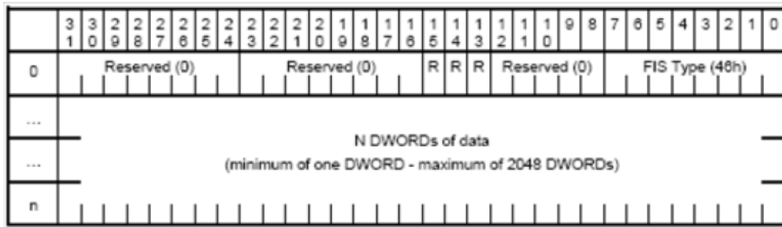
Data FIS layout
