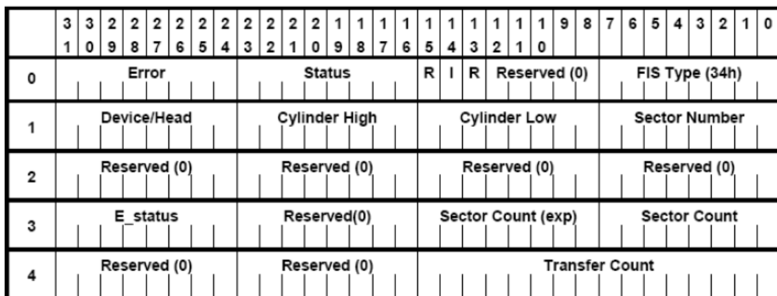
PIO Set up layout (CHS mode: Commands include PIO data transfer)
