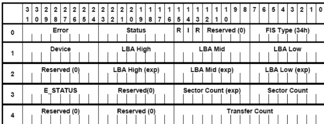
PIO Setup layout (48bit LBA mode: Read/Write Sector EXT)
